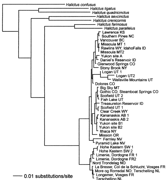
FIG. 3. The maximum-likelihood tree indicating branch lengths. FR, France; NO, Norway; NL, the Netherlands; SW, Switzerland; AB, Alberta, Canada.
